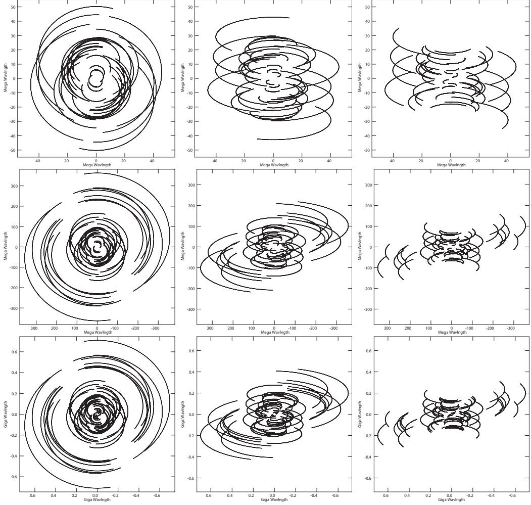
Figure 3: Examples of (u, v) coverage for an EAVN observation with full array configuration in the 2023B semester at C-band (upper panels), K-band (middle panels) and Q-band (lower panels) with the source's declination of +60^\circ (left panels), +20^\circ (center panels), and -20^\circ (right panels). Total observation duration of 10 hours and the antenna's lower elevation limit of 15^\circ are assumed for all cases.
