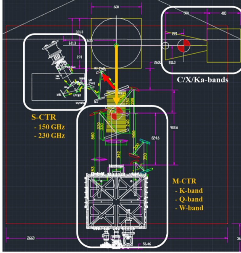
Figure 14: The CTR receiving system installed on the KPC.
